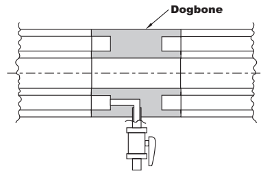
Figure G-11. Containment Pipe: Duo-Pro® and Fluid-Lok®
